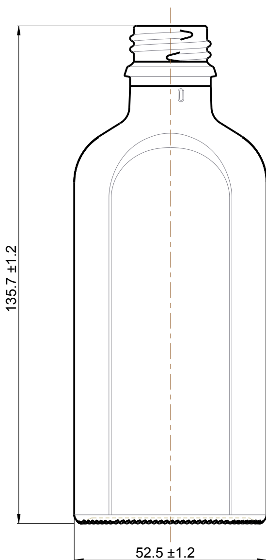
Front view GL 22x3
